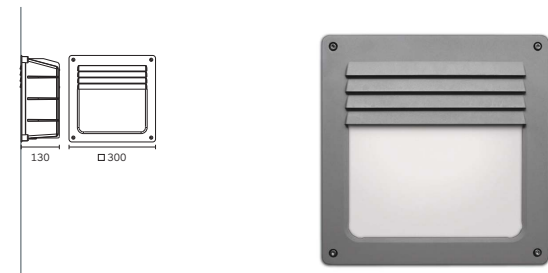
Scudo Ramp Glass Diffuser + Grid Wall Recessed
