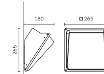
Scudo Wall Polycarbonate diffuser Fixed Surface Mounted
