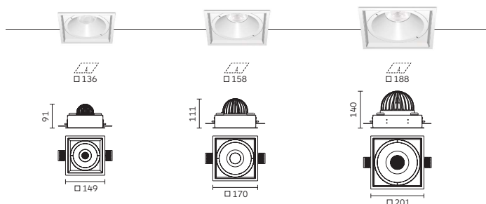
Palla 70 / 100 / 130 Fixed Square Trim
