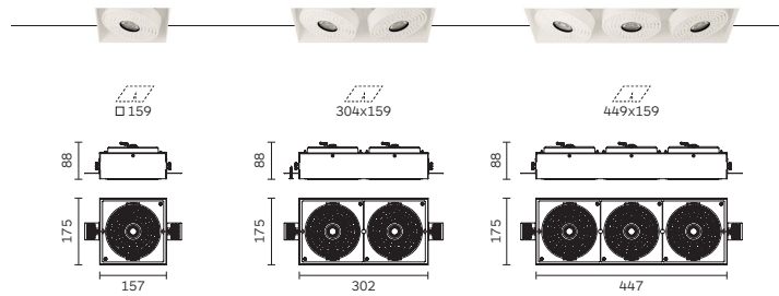
MultiArena 130 Adjustable Trimless
