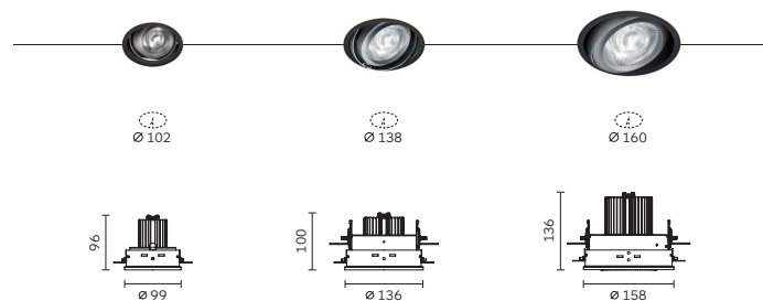
Gimbalo 60 / 100 / 130 Adjustable Trimless
