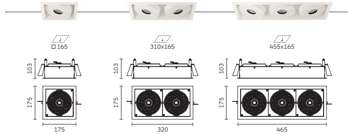
MultiArena 130 Adjustable Trim
