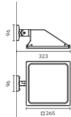
Scudo Wall with Glass diffuser Adjustable Surface Mounted
