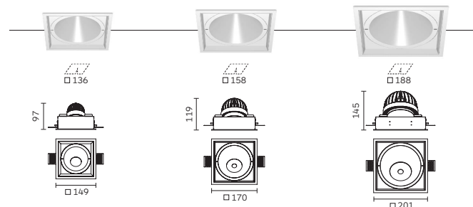
Palla 70 / 100 / 130 Wallwasher Square Trim
