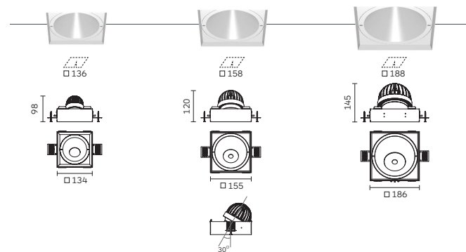
Palla 70 / 100 / 130 Wallwasher Square Trimless
