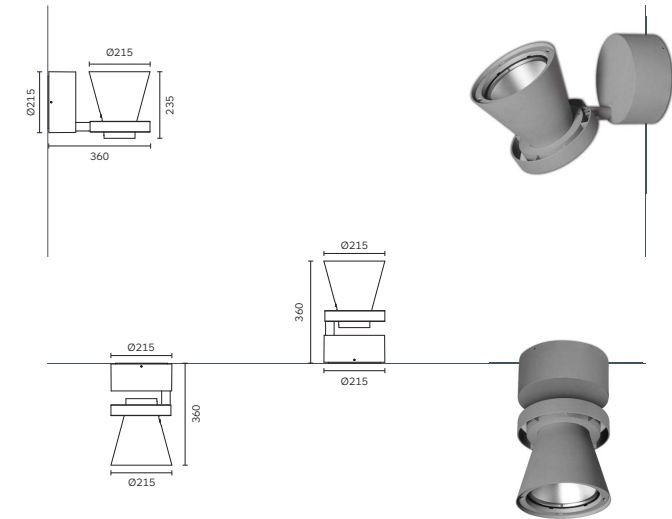
Galileo Due 215 Ceiling/Ground Surface mounted
