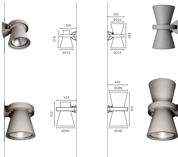
Galileo 215 Up or Down / Up & Down Surface mounted
