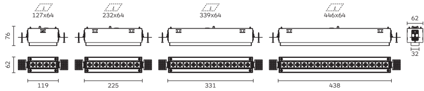
Polaris 30 Adjustable Trimless
