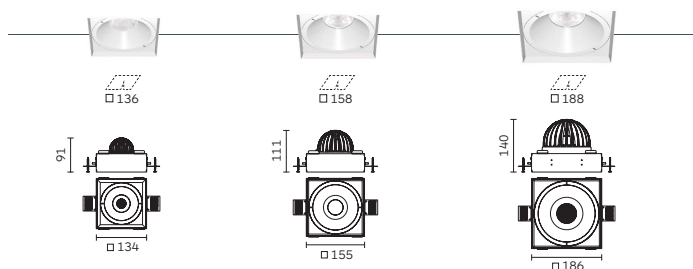
Palla 70 / 100 / 130 Fixed Square Trimless
