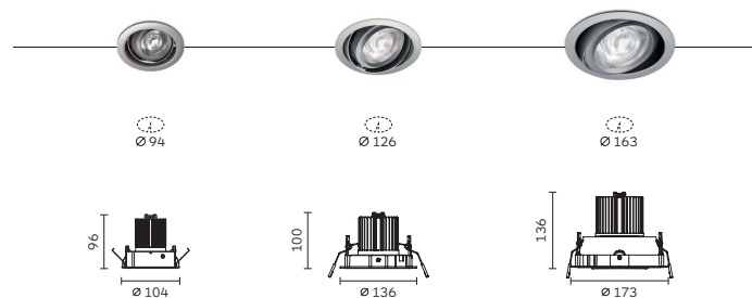
Gimbalo 60 / 100 / 130 Adjustable Trim
