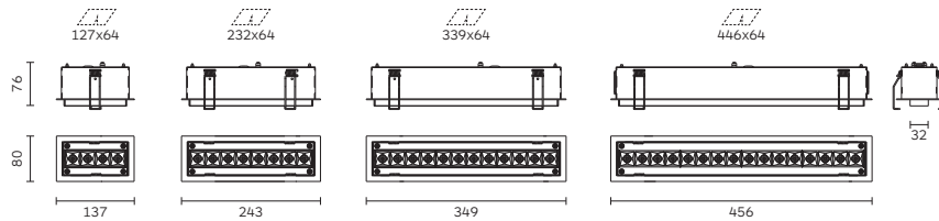
Polaris 30 Adjustable Trimless
